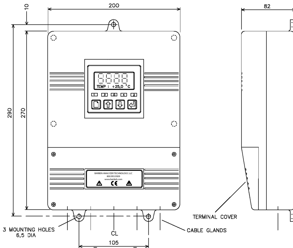
Figure 1 : Overall dimensions MSSD53.
