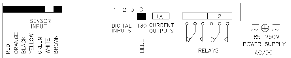
Figure 3: MSSD53 Terminal connections.
