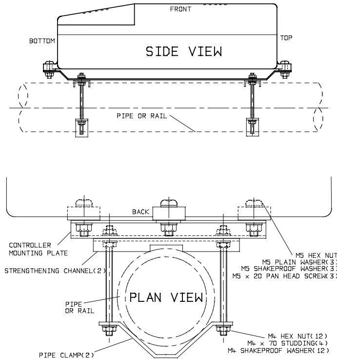
Figure 2: MSSD53 handrail & pipe mounting brackets.
