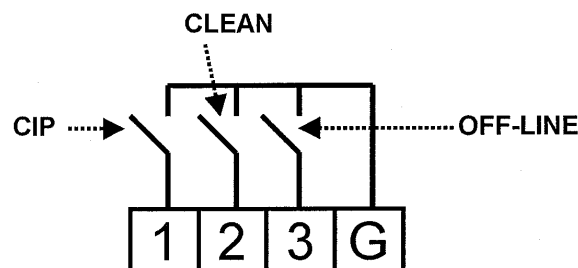
Figure 7: Digital Inputs
